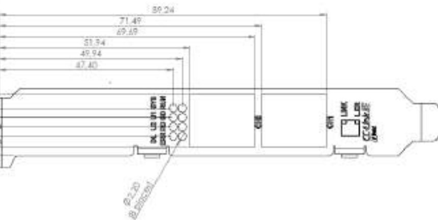
Figure 71: Dimensions Front Panel CIFX 50E-CCIES
